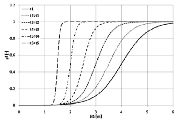
Figure 5. Contraction of the capsize rate with increased time of observation (Papanikolaou et al., 2013)
