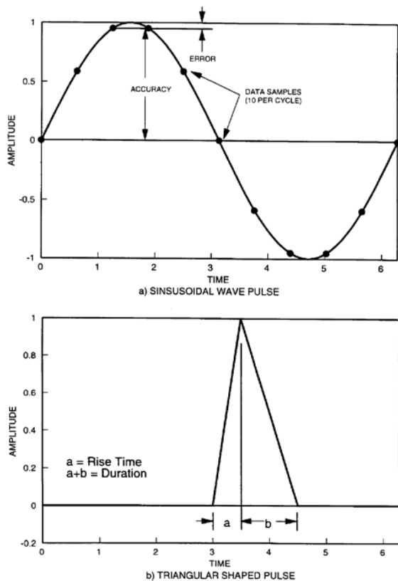
Figure 8. Examples of Loading Time Histories as Relates to Required Sample Rates (Dinsenchacher, 2010).
