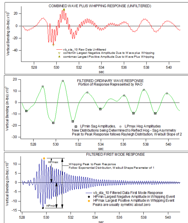
Figure 10. Example of Analysis to Filter and Arrive at First Mode and Whipping Responses (Dinsenbacher, 2010).
