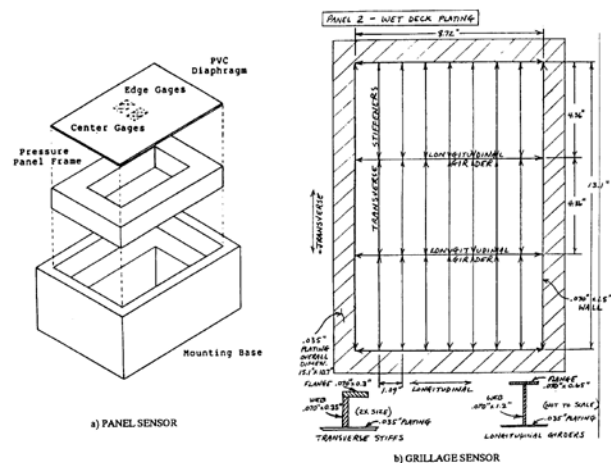
Figure 9. Example of Panel and Grillage Sensors (Dinsenchacher, 2010).
