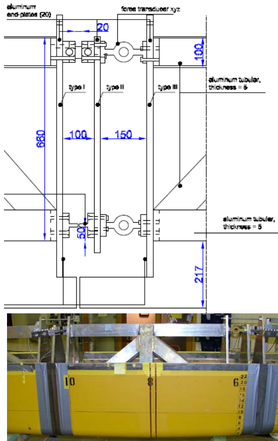
Figure 5. Instrumented Flexible Connections for Non-Backbone Elastic Segmented Model (Drummen, 2007).
