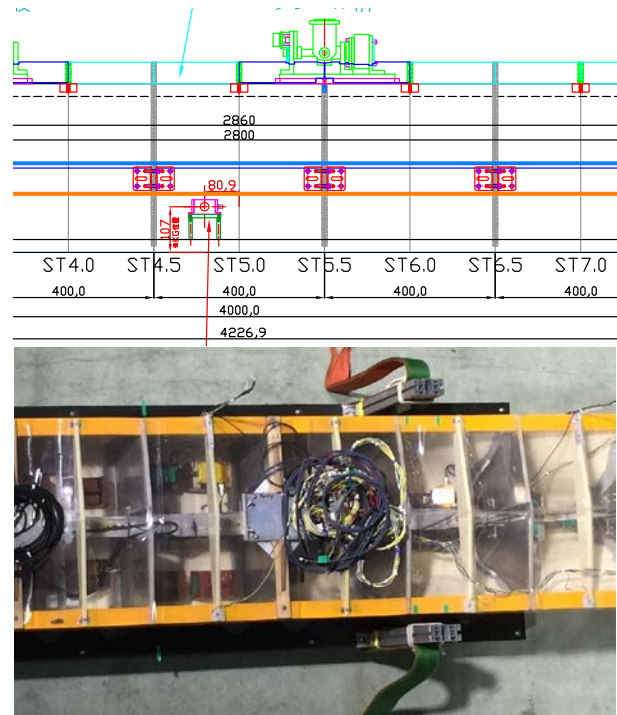
Figure 1. Elastic Segmented Model with Internal Backbone Beam (Miyake, 2009).
