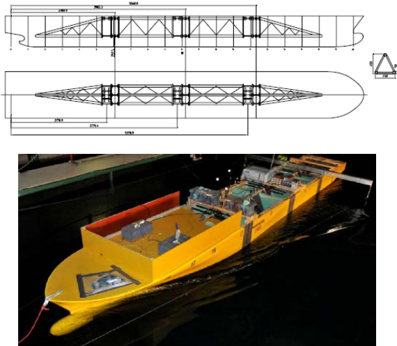
Figure 2. Segmented Elastic Model with Transducers at Segments (Wu, 2010).
