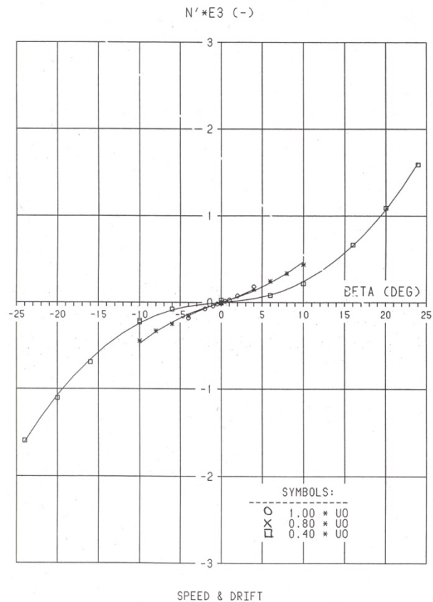
Figure 1: Comparison of measured and predicted yaw moment. Lines indicate simulation model
