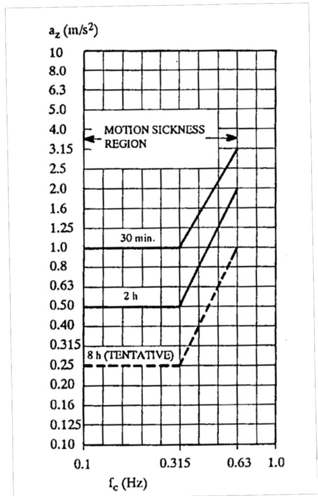
Fig.1. ISO 2631/3 Severe Discomfort Boundaries
