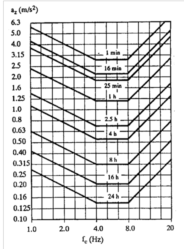
Fig. 2. ISO 2631/1 Fatigue-Reduced Proficiency Boundaries
