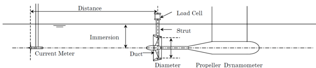
Figure 3 Typical Set Up for Tests on Ducted Propellers in a Towing Tank
