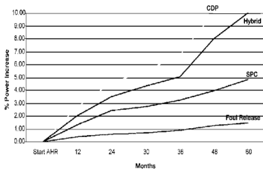
Figure 2: Overall % power increase for a typical fast fine ship (e.g. Container Liner) vs. time for different antifouling types
