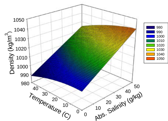
Figure 9: Seawater density
