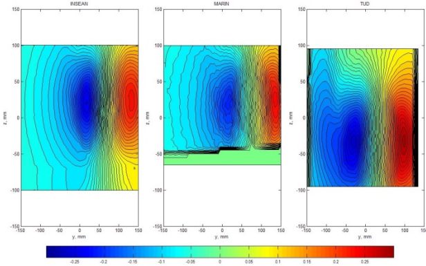
Figure 19: W velocity contours at the P2 plane. The order of images (from left to right) is INSEAN, MARIN and TUD.
