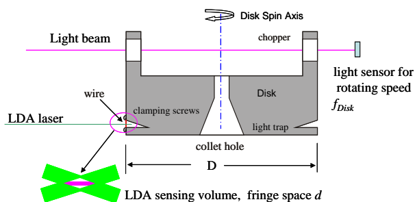
Figure 5: Spinning wire schematic at NIST by Yeh and Hall (2007)
