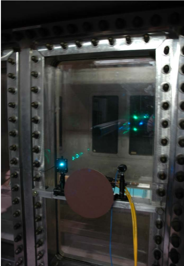
Figure 6: Photograph of a focused 4-beam probe
