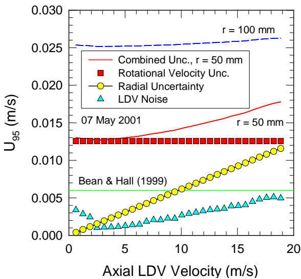
Figure 3: Absolute velocity uncertainty of rotating disk with r = 50 mm
