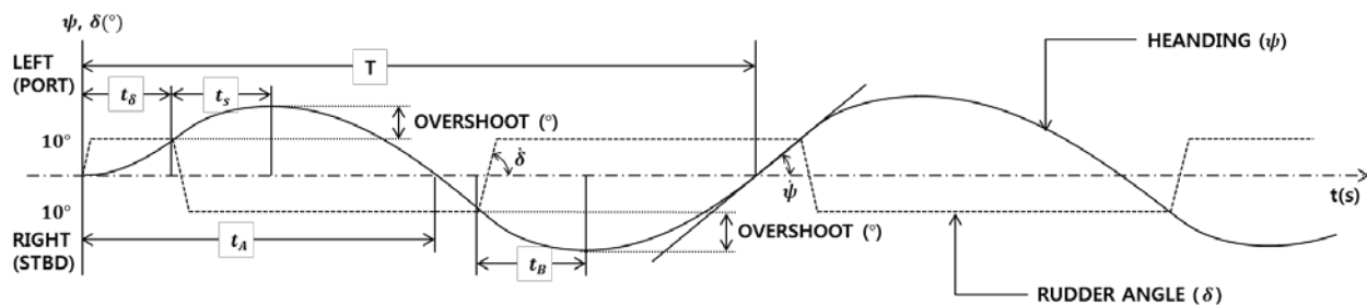
Figure 2. Time trace of zigzag manoeuvre parameters
