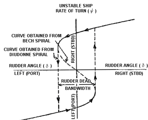
Figure 3: Presentation of spiral manoeuvre results
