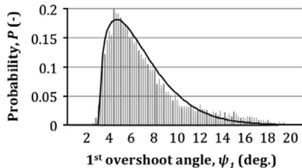
Figure F5: probability distribution of the obtained first overshoot angles after Monte Carlo simulations (Woodward, 2014).
