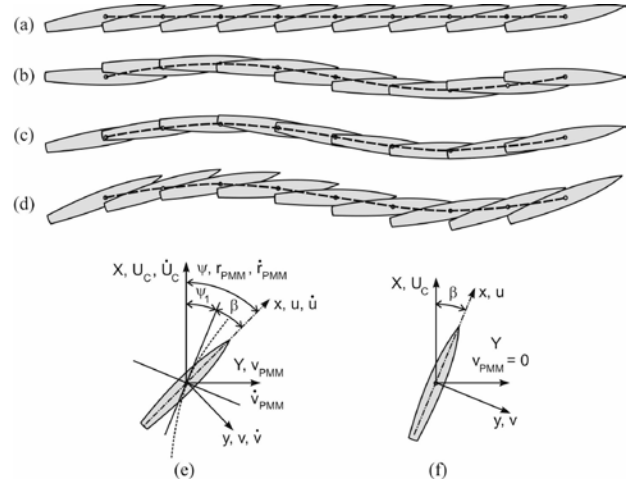
Figure A6 Definitions of PMM tests and motion parameters: (a) static drift; (b) pure sway; (c) pure yaw; (d) yaw and drift; (e) dynamic test motion parameters; (f) static test motion parameters.
