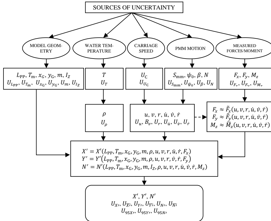
Figure A7 Sources of uncertainties in a PMM test.
