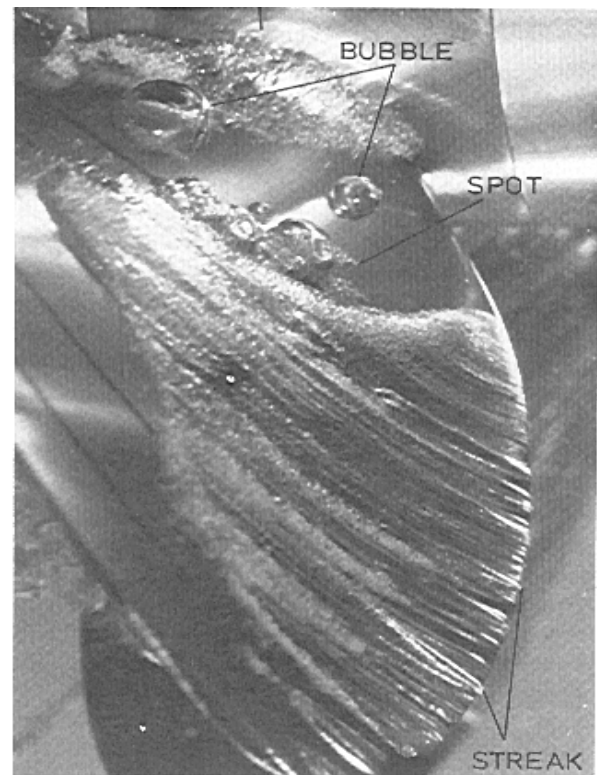
Figure 2 Leading edge, large bubble and root cavitation
