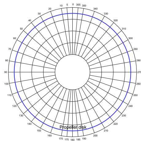
Fig. 11 Measurement grid for wake measurement
