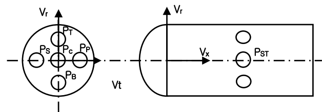
Figure 2 Position of the pressure holes
