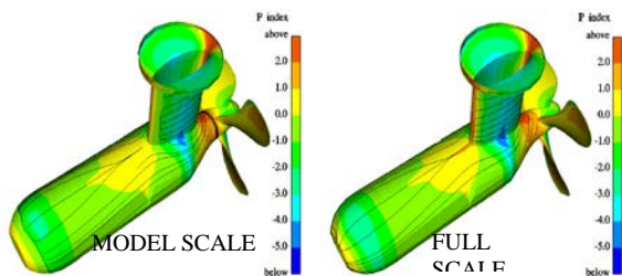
Figure 15 Pressure distributions and streamlines on pod housing/strut surfaces at model and full scale (Sanchez-Caja, et al. 2003)
