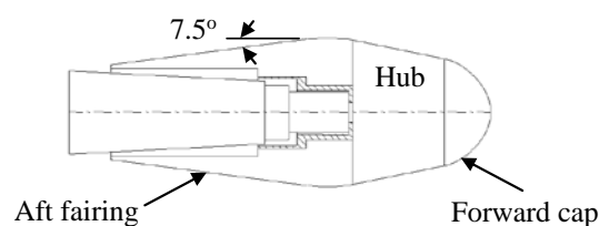
Figure 2 Example of hub geometry for an open water test with a pulling type propeller.
