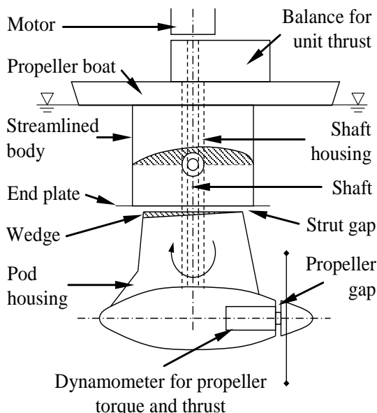
Figure 4 Typical pod unit open water test set-up
