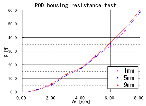
Strut gap Figure.8 Pod resistance of table 4 with different strut gaps
