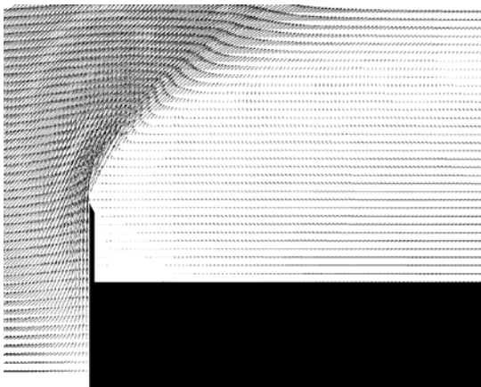
Figure 4 Velocity vectors around the fence
