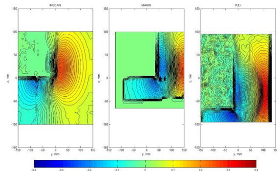
Figure 16: W velocity contours at the P1 plane. The order of images (from left to right) is INSEAN, MARIN and TUD.
