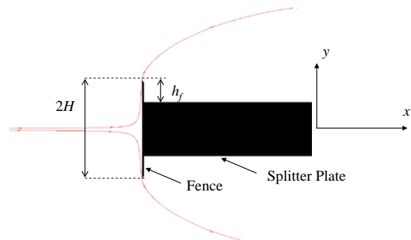
Figure 2 Geometry of the 2D benchmark
