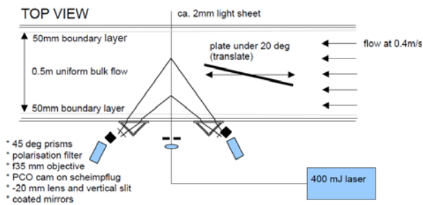
Figure 13: Sketch of TUD's stereo PIV setup in a circulating water tunnel.
