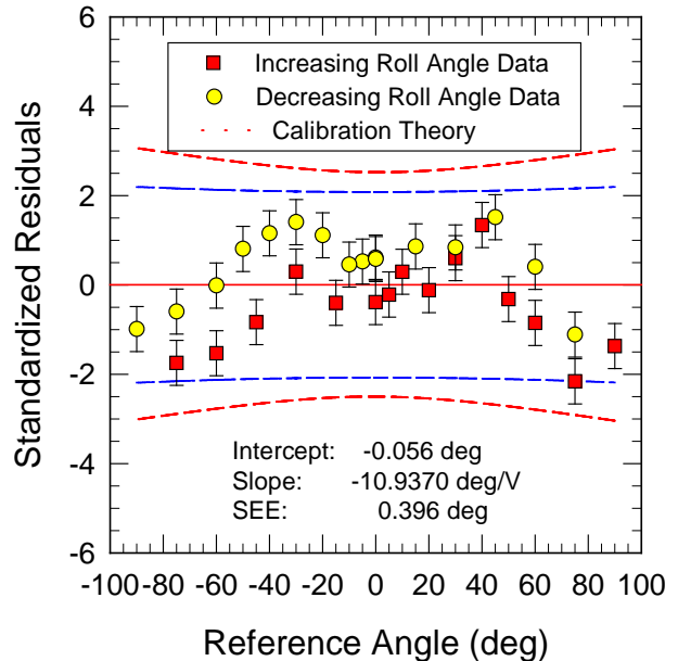
Figure 3c: Calibration Data for Vertical Gyroscope in Roll - Standardized Residuals
