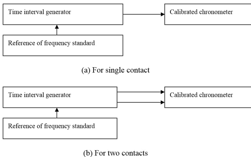
Fig. 4 The instruments connection diagram of the action time measurement of the mechanical contacts
