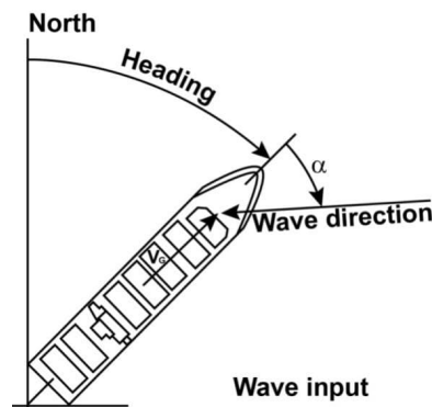
Figure 5. Sign convention for wave directions
