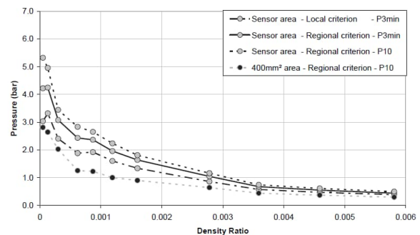
Figure 3: Pressure results vs. density ratio for several criteria of post-processing (Maillard and Brosset (2009))
