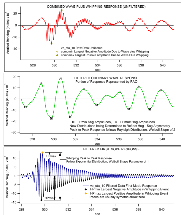
Figure 11. Example of Analysis to Filter and Arrive at First Mode and Whipping Responses (Dinsbacher, 2010).
