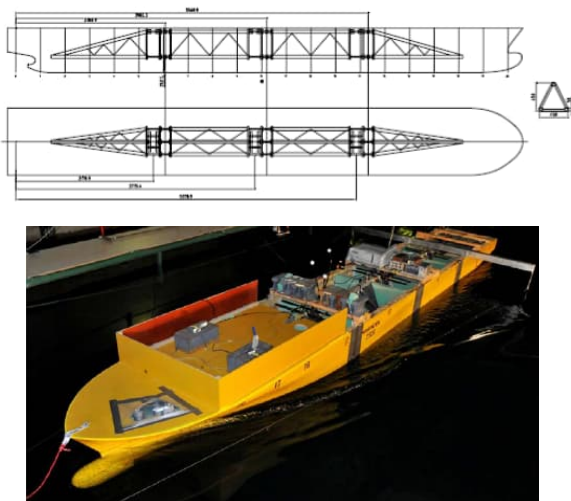
Figure 3. Segmented Elastic Model. Rigid segments with flexible connections and transducers between the segments (Wu, 2010).
