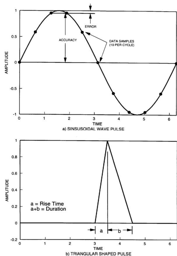
Figure 9. Examples of Loading Time Histories as Relates to Required Sample Rates (Dinsenbacher, 2010).
