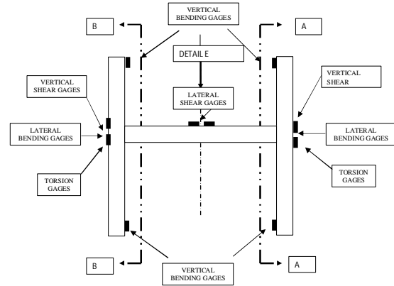
Figure 5. Possible Strain Gage Measurement for Internal Elastic Strength Bar (Dinsenbacher, 2010).
