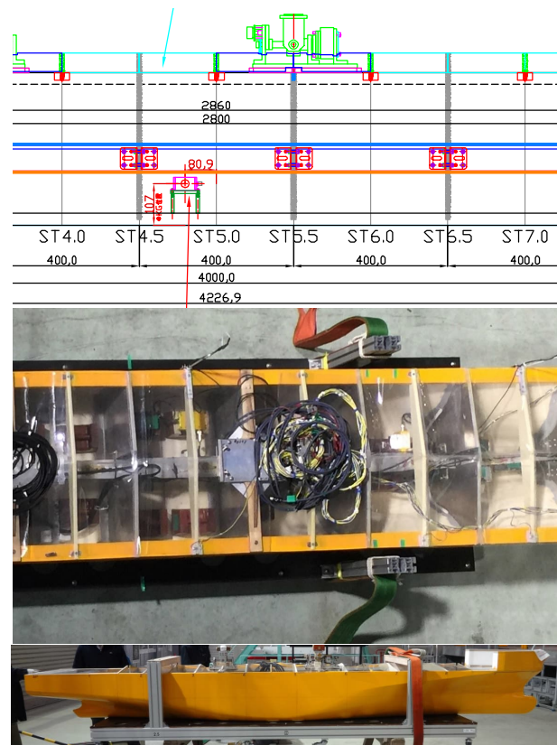
Figure 4. Hydro-structural model with backbone (Houtani, 2016).
