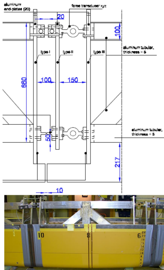
Figure 6. Instrumented Flexible Connections for Non-Backbone Elastic Segmented Model (Drummen, 2007).
