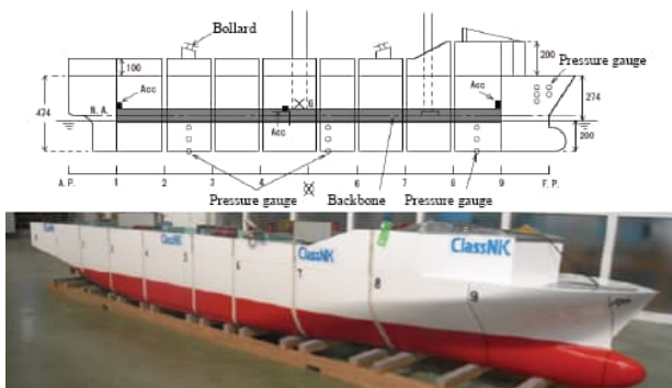
Figure 2. Elastic Segmented Model with Internal Backbone Beam (Miyake, 2009).
