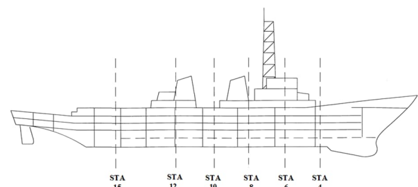
Figure 7. Example Segmentation Spacing (Din-senbacher, 2010).
