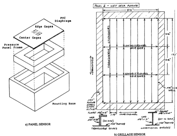
Figure 10. Example of Panel and Grillage Sensors (Din-senbacher, 2010).
