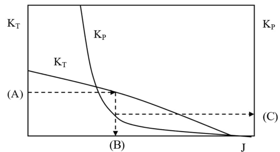
Figure 6: Propeller Open Water Chart (TNM)
