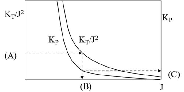
Figure 7: Propeller Open Water Chart (RTIM)
