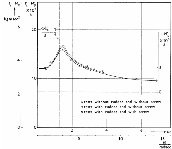
Figure 5: Influence of \omega'_3 on added moment of inertia from PMM yaw tests (van Leeuwen, 1964)
