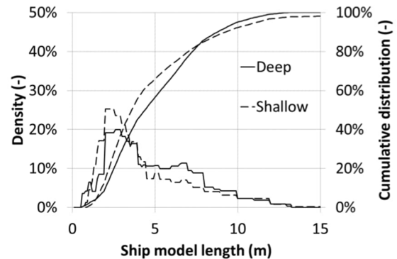
Figure 1: Influence of water depth on ship model length distribution.
