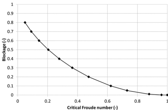
Figure 3: Effect of the blockage on the critical Froude number.
