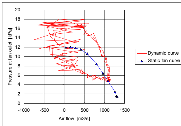
Figure 1 – Differences in the pressure flow relation if compared to static measurements experienced at MARIN on a captive model of a SES.
