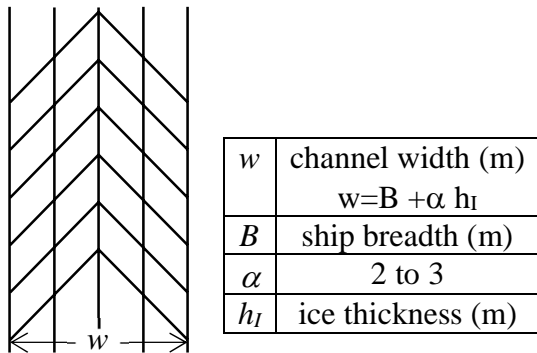
Figure 5: An example of pre-sawn cutting pattern
