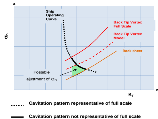
Figure 5: Cavitation inception diagram with isolated vortex cavitation at model-scale.
