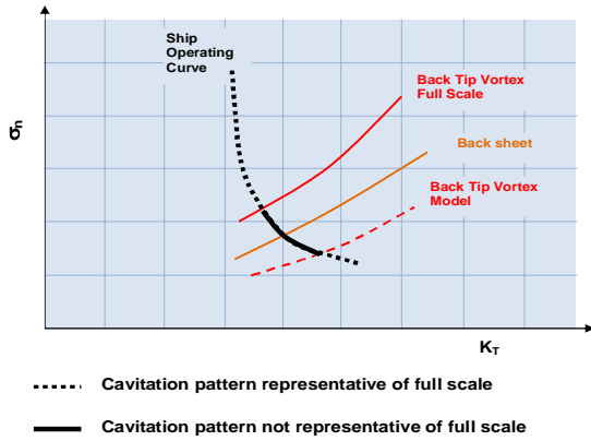
Figure 6: Cavitation inception diagram with no isolated vortex cavitation at model-scale
