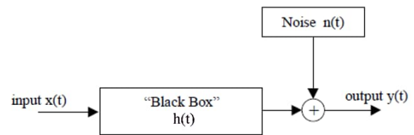
Figure 3: Scheme of input/output system (Tani et al. , 2016b).
