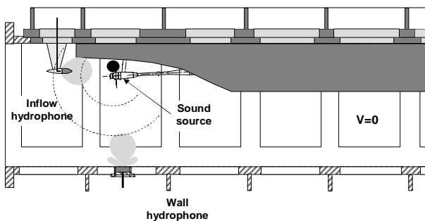
Figure 2: Transfer function measurement set-up in cavitation tunnel
