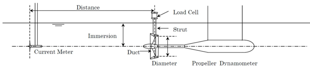
Figure 3 Typical Set Up for Tests on Ducted Propellers in a Towing Tank
