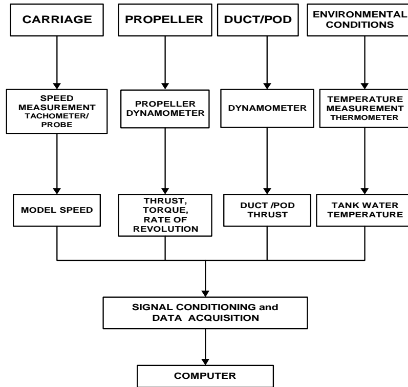
Figure 4 Typical Measurement System
