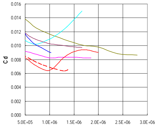
Figure 14 Drag Coefficients (Cd) measured by 7 model basins
