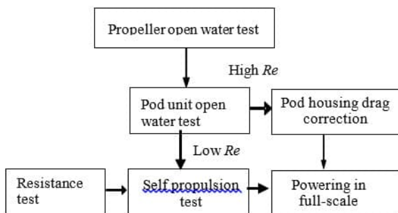
Figure 1 Flow diagram of power prediction of a vessel with podded propulsion systems
