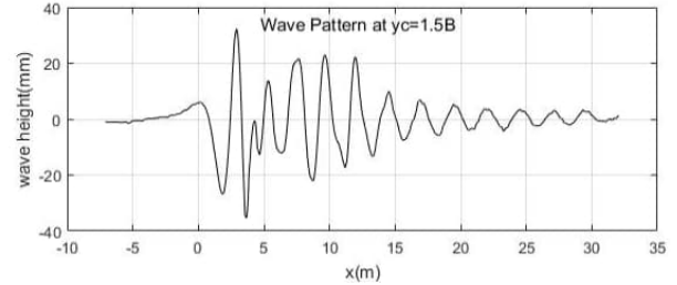
Figure 4 Measured wave height curve at y_c = 1.5B
