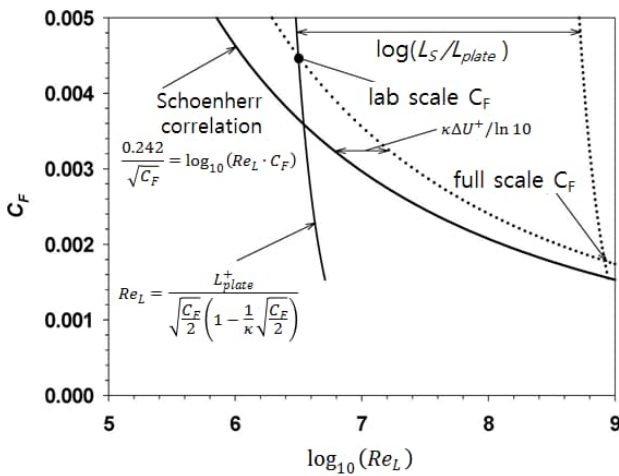
Fig. 1 Graphical representation of Granville’s similarity law scaling
