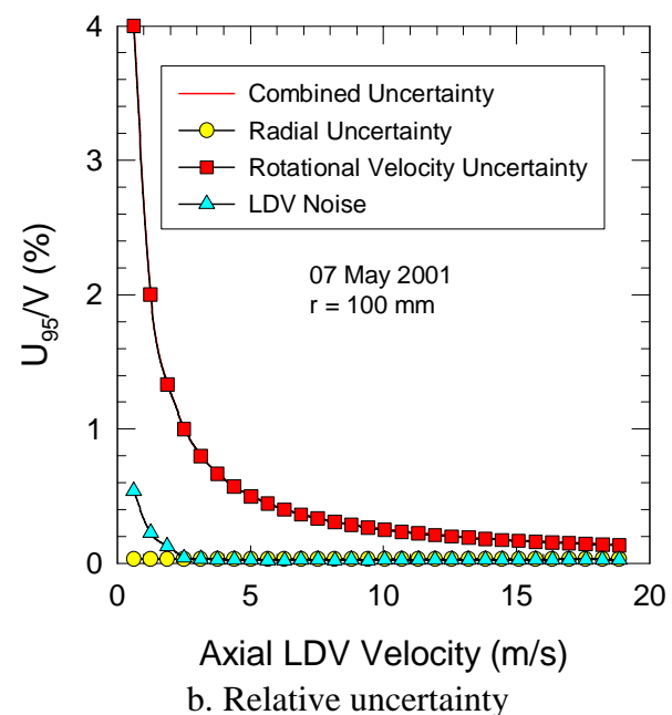
Figure 2: Velocity uncertainty of rotating disk for r = 100 mm
