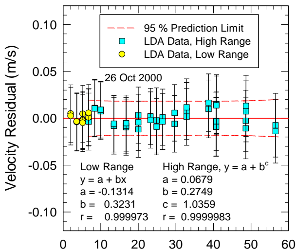
Figure 5c: Calibration data for water tunnel speed in empty test section - residual plot for non-linear curve
