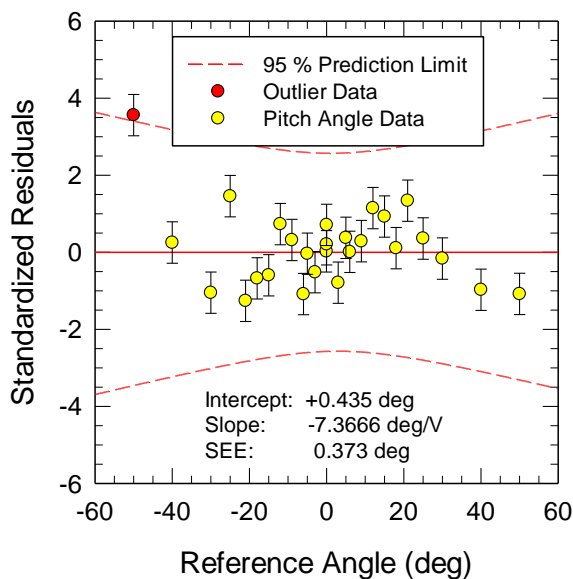
Figure 4b: Calibration data for vertical gyro-scope in pitch - Standardized residuals
