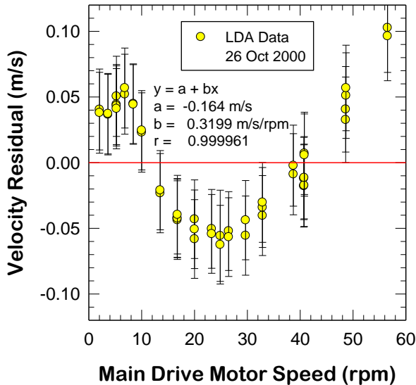
Figure 5b: Calibration data for water tunnel speed in empty test section - residual plot for linear curve
