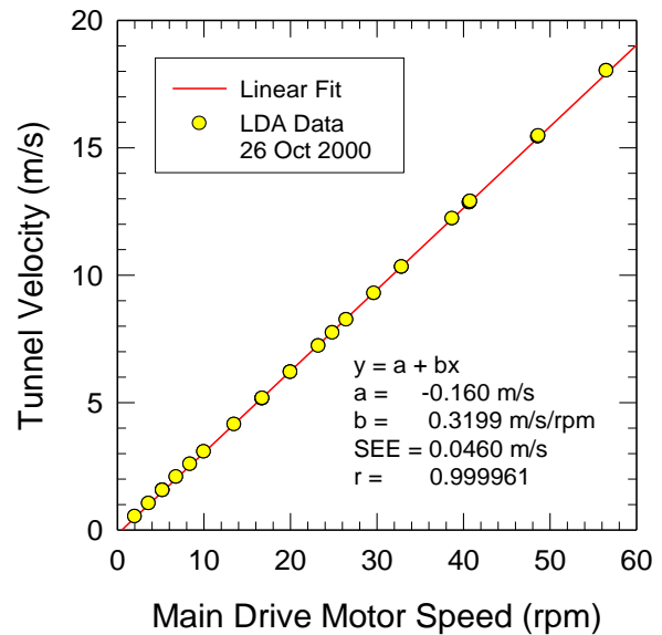
Figure 5a: Calibration data for water tunnel speed in empty test section - linear plot
