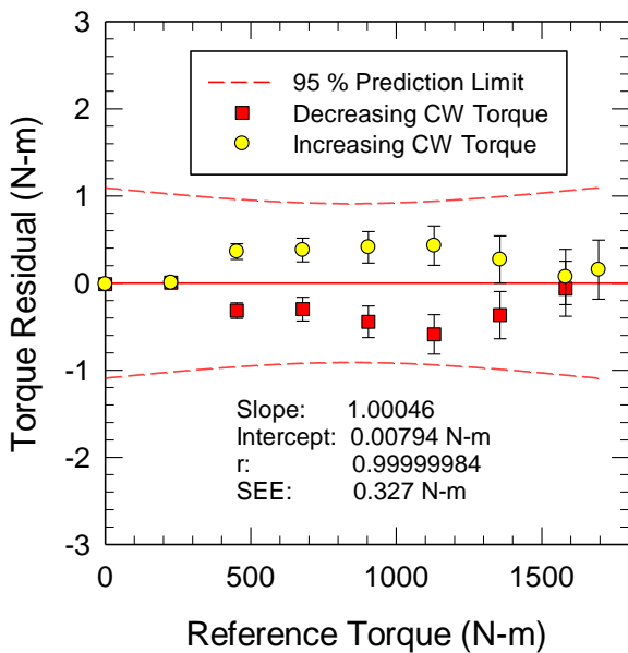
Figure 6b: Calibration data for commercial torque cell - residual plot
