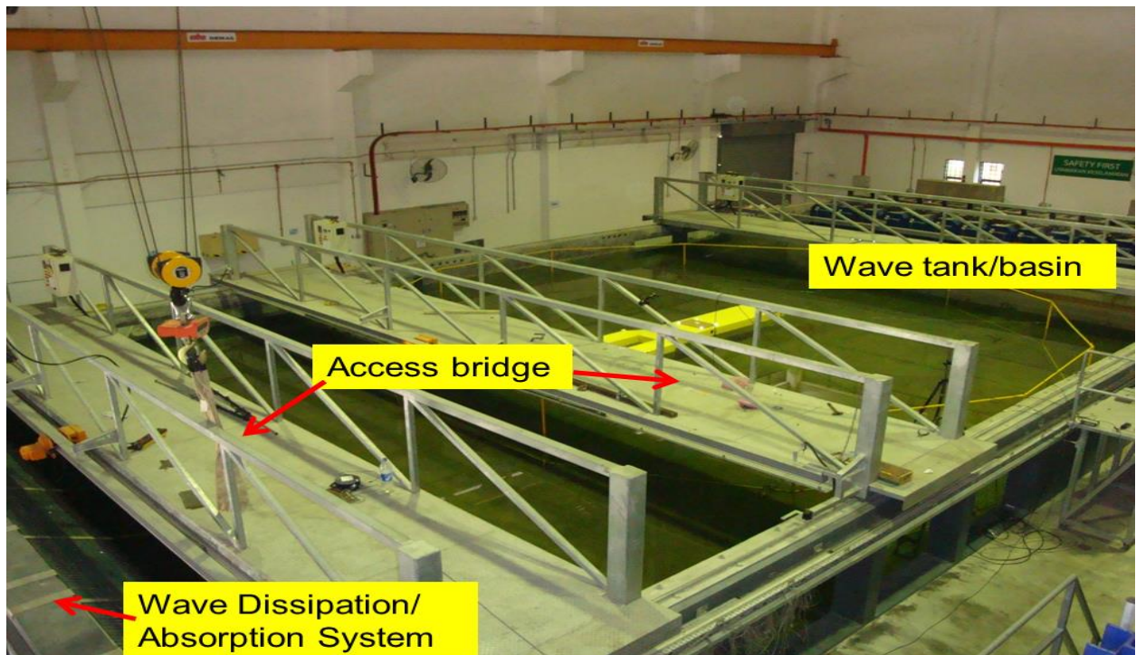
Figure 2: Wave Basin Photo
