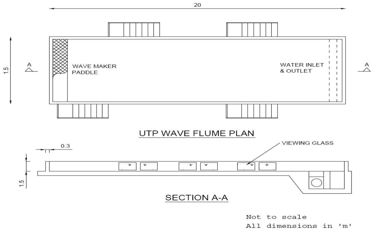
Figure 3: UTP Wave Flume
