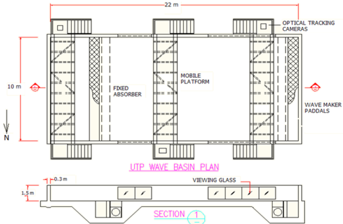
Figure 1: UTP Wave Basin
